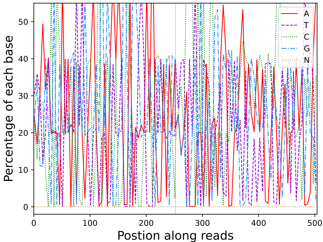
Base percentage along reads (R10412)
